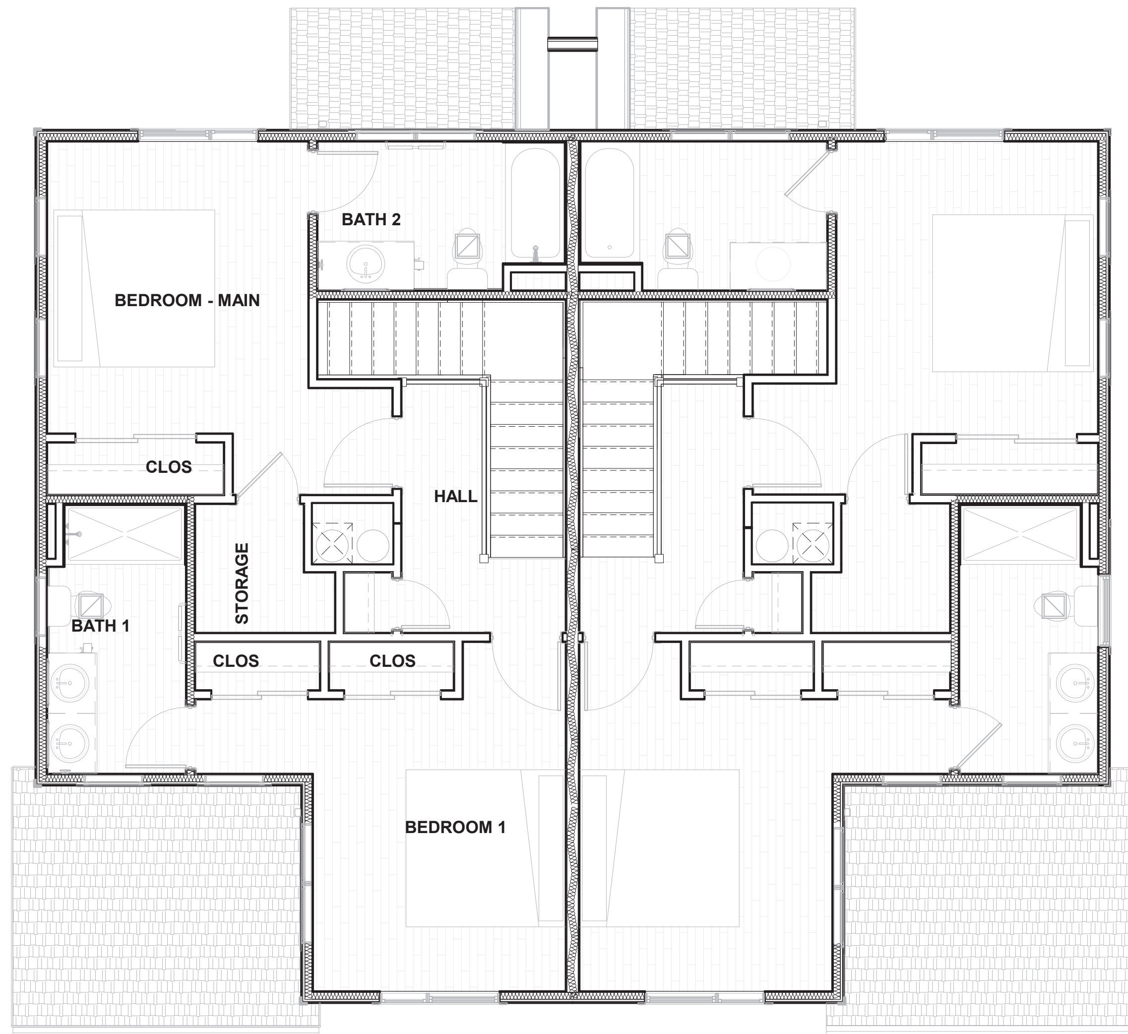
② Second Floor - Pulley 1/4" = 1'-0"
