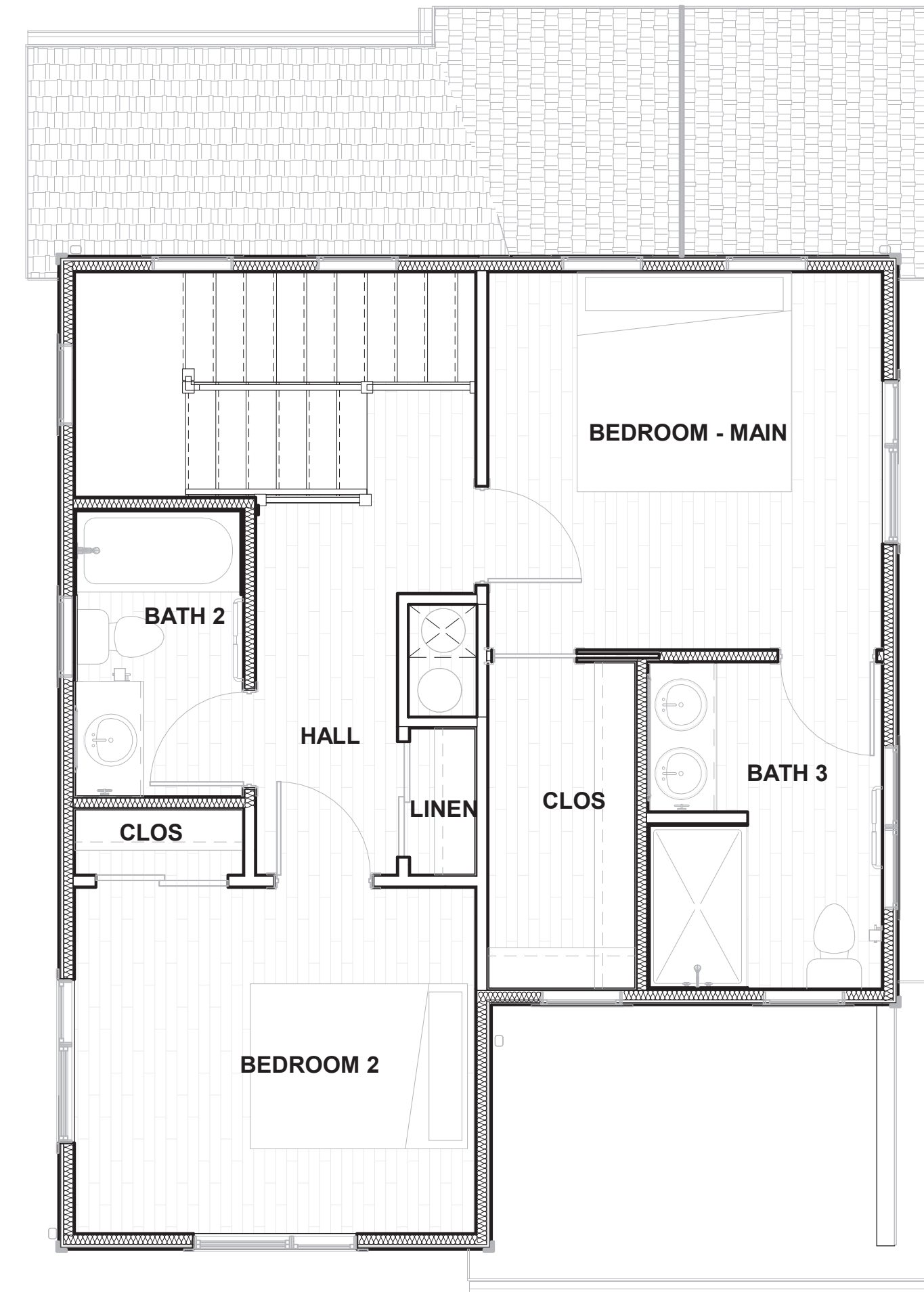
② Second Floor - Jones 1/4" = 1'-0"
