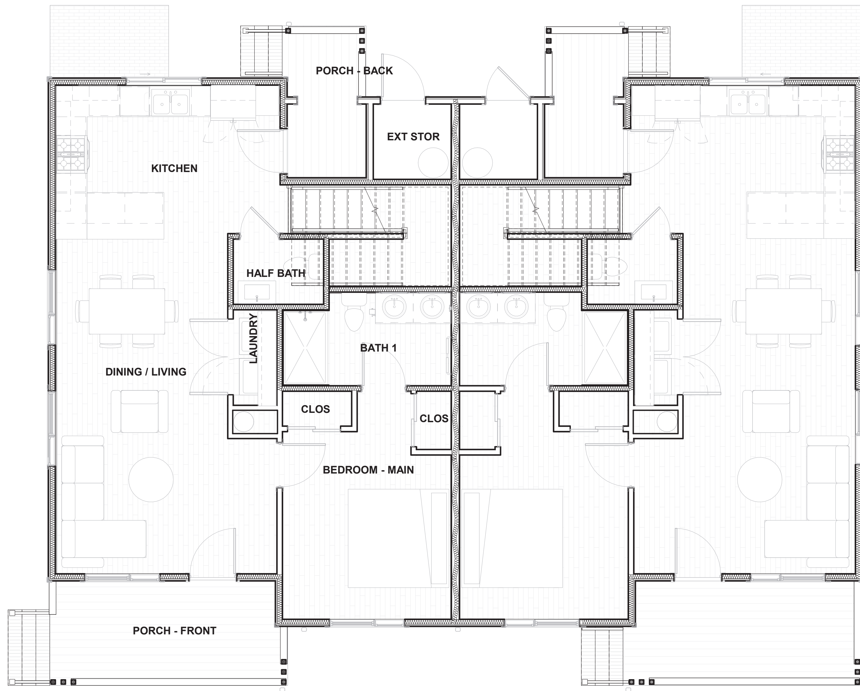
① First Floor - McDougald 1/4" = 1'-0"
