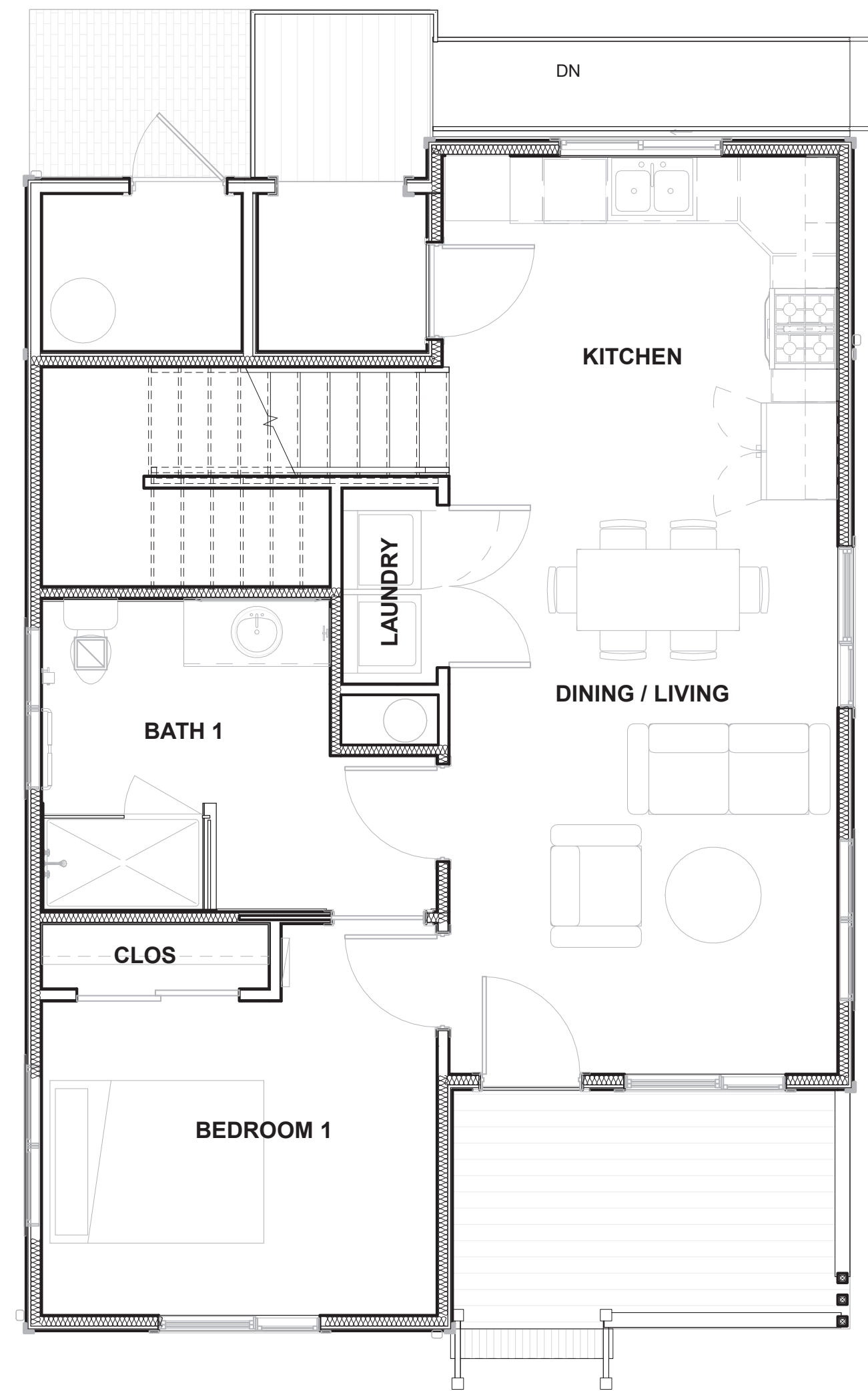
① First Floor - Jones 1/4" = 1'-0"
